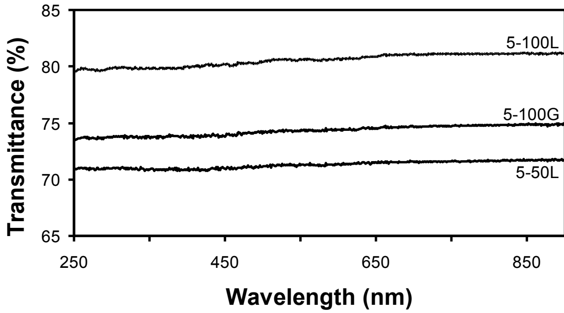
Figure 4. Optical transparency of 5-100G, 5-100L, and 5-50L CG-OTEs.
