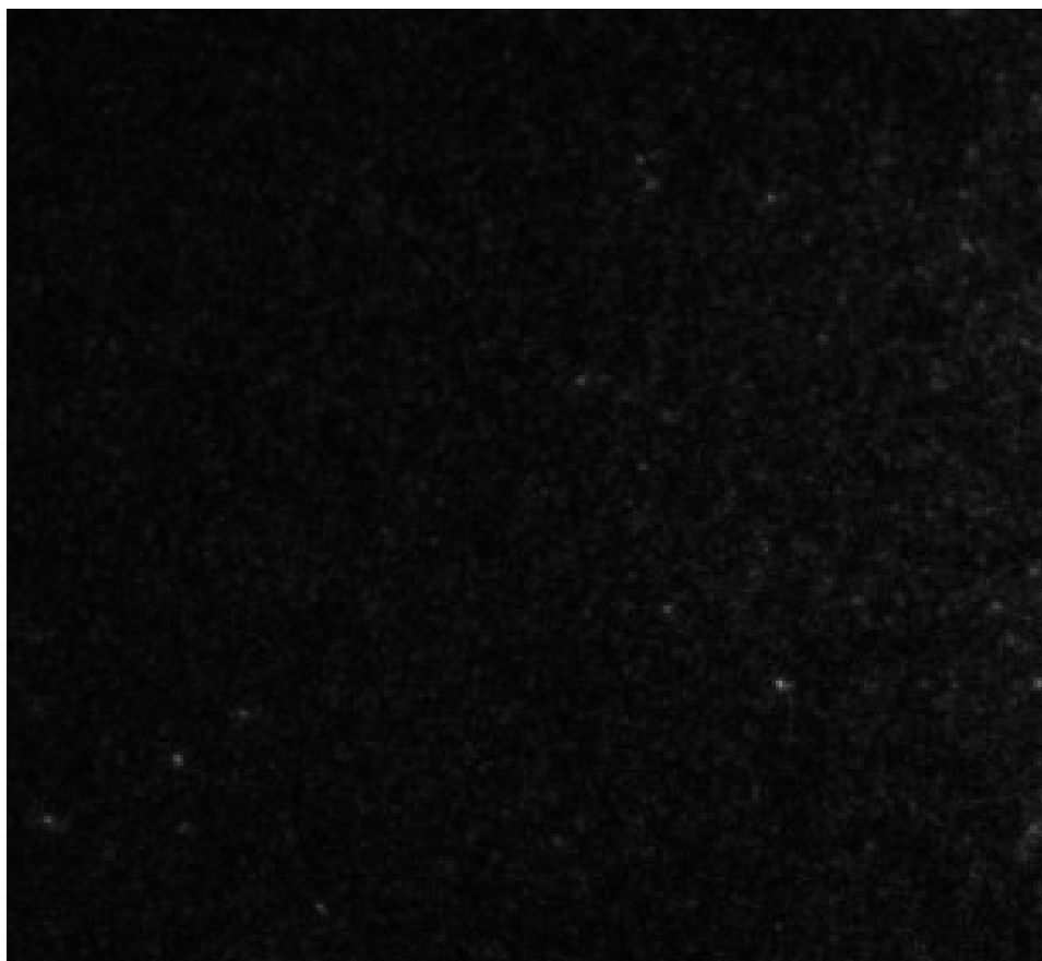
Figure 3b. Desorption and repulsion of HPV-16 molecules from new C-OTE with E_{app} = -2.0 V.
