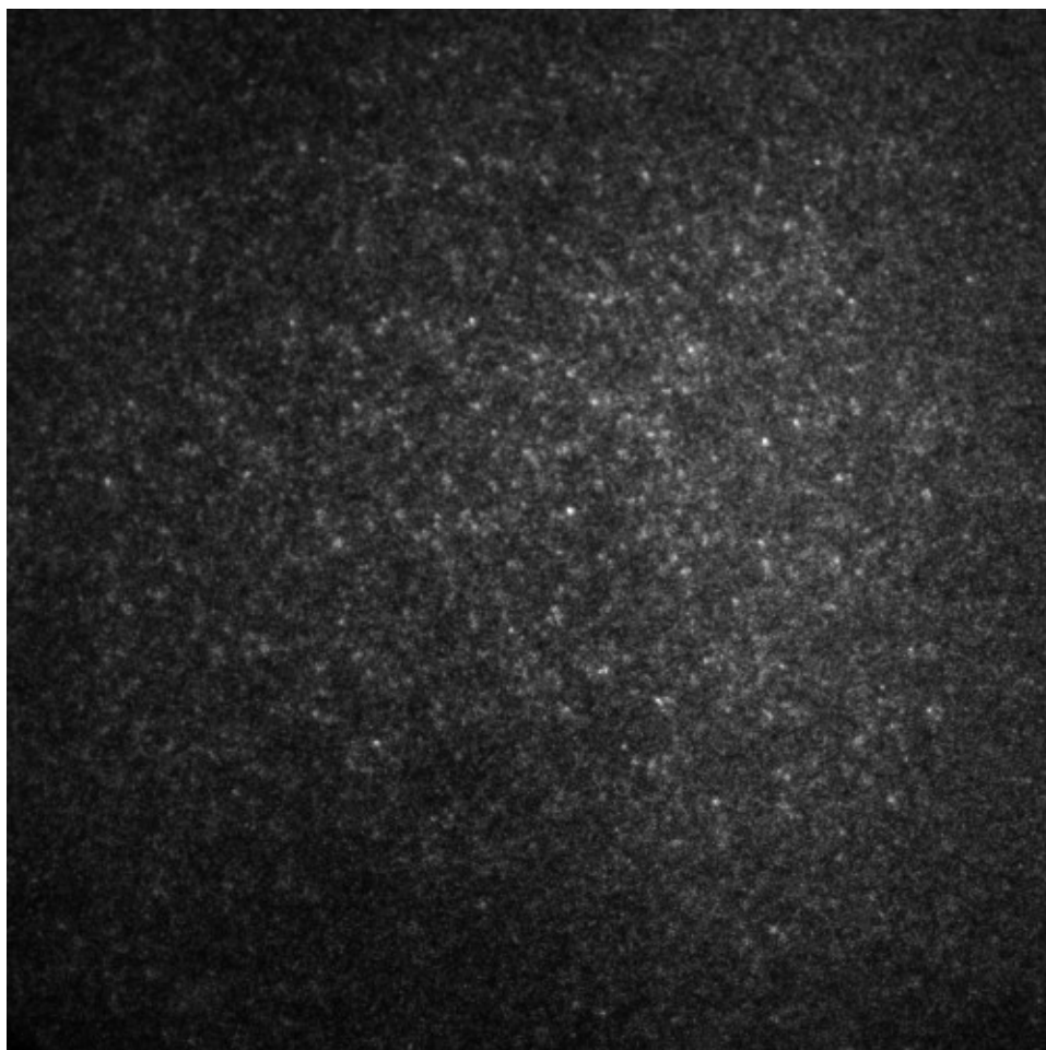
Figure 4c. Fluorescence of 1 kbp DNA within 120 nm of C-OTE at E_{app} = +1.0 V.
