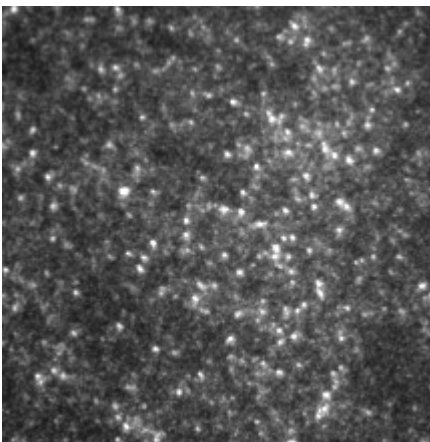
Figure 4h. Close-up of figure 4g. Fluorescence of 1 kbp DNA within 120 nm of C-OTE at E_{app} = +2.0 V.
