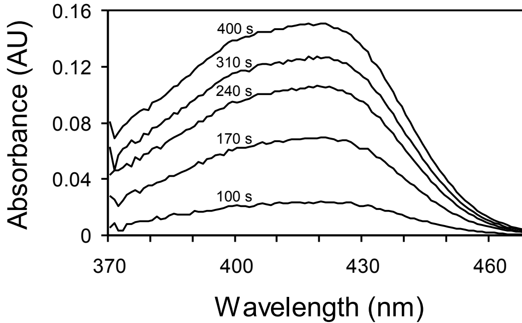
Figure 6. Absorbance of ferricyanide over time after the potential applied to a 10.0 mM solution of ferrocyanide (1.0 M KCl) is stepped to +600 mV (vs Ag/AgCl, sat'd KCl) at a 5-100G CG-OTE.
