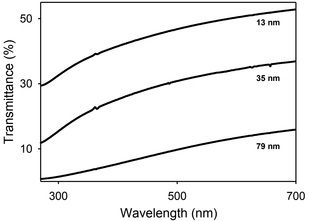
Figure 2. Optical transmittance of C-OTEs as a function of wavelength for three different pyrolyzed film thicknesses (13, 35, and 79 nm).
